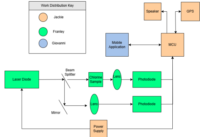
Fig. 1. A hardware block diagram that shows the flow of data, connections, and communication.
