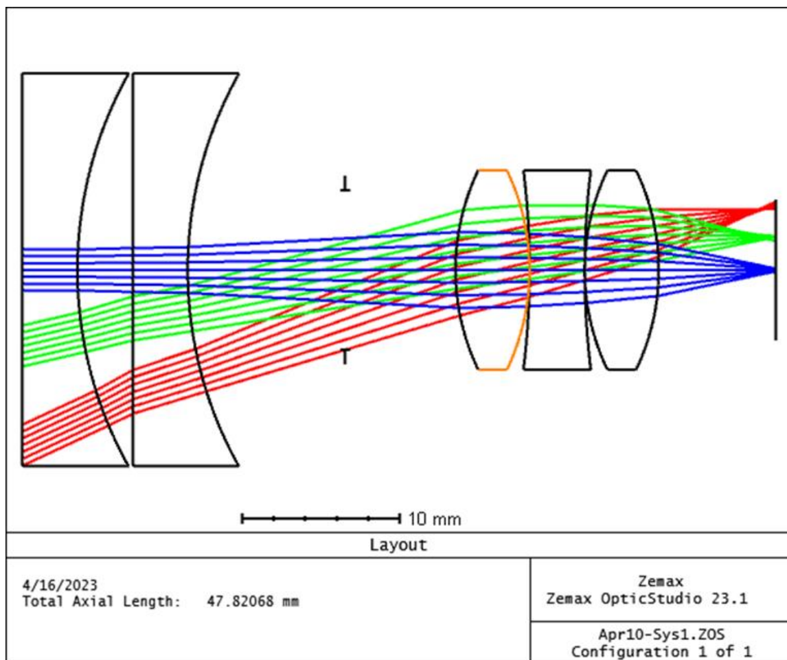
Figure 48: Zemax ray trace of final system
