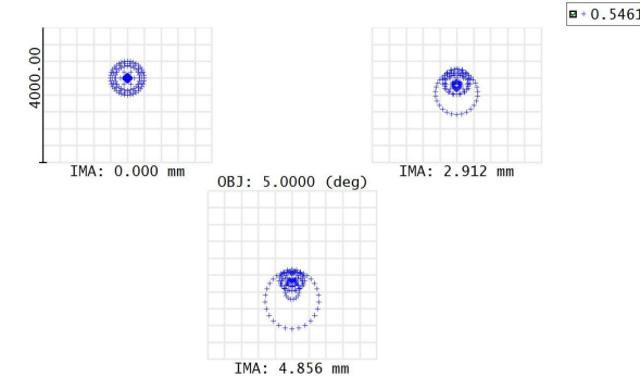
Fig. ###. (Above) Total Optical Design in Zemax, (Below) Spot Size Diagram for on and off axis rays at various points along the path length.
