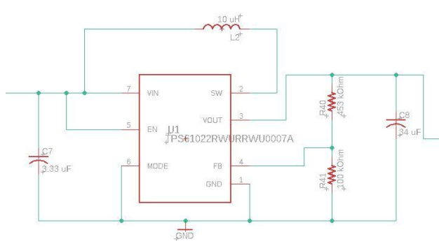
Fig. 5. Circuit schematic for the 5-volt to 3.3-volt voltage regulator.
