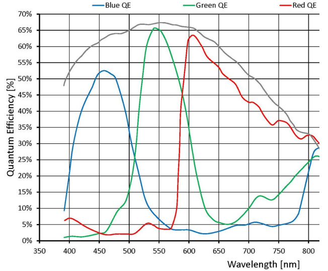
Fig. 2. Quantum efficiency of the Alvium 1500 C-120 camera. [2]
