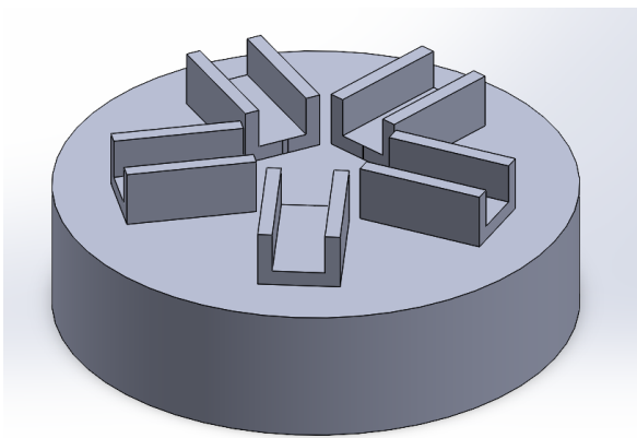
Fig. 11. Image and design of the tray.
