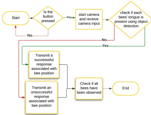
Fig. 10. Object detection flowchart.
