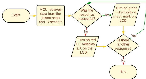
Fig. 7. LED/LCD flowchart.
