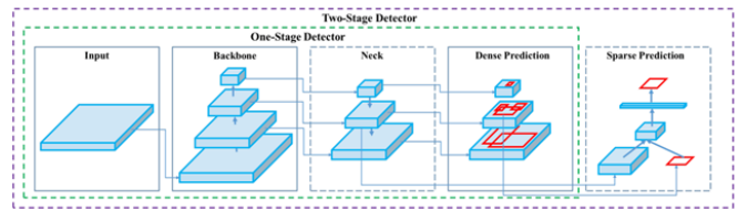
Fig. 9. Structure of the YOLOv4 model. [4]
