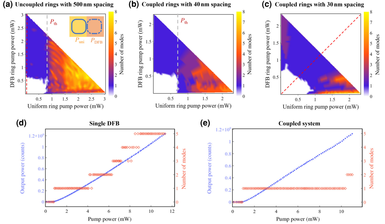
FIG. 4. (a)–(c) Number of lasing modes as a function of pumping intensities of the ordinary uniform ring ( P_{uni} ) and the DFB ring ( P_{DFB} ). The measurements are performed for samples with the spacing between rings of (a) 500 nm, (b) 40 nm, and (c) 30 nm. Gray dashed lines indicate the lasing threshold of the uniform ring. The upper right inset of (a) shows what takes place in the measurement while pumping at various powers for each ring. (d), (e) Output power and number of lasing modes versus pump power for (d) the single DFB ring and (e) the coupled system. The plots of the number of modes in (d), (e) correspond to the cross-sectional views of the color map sliced by the red dashed lines in (a), (c), respectively. The lasing thresholds ( P_{th} ) of the single DFB and the coupled system are similar at 0.76 and 0.97 mW, respectively.
