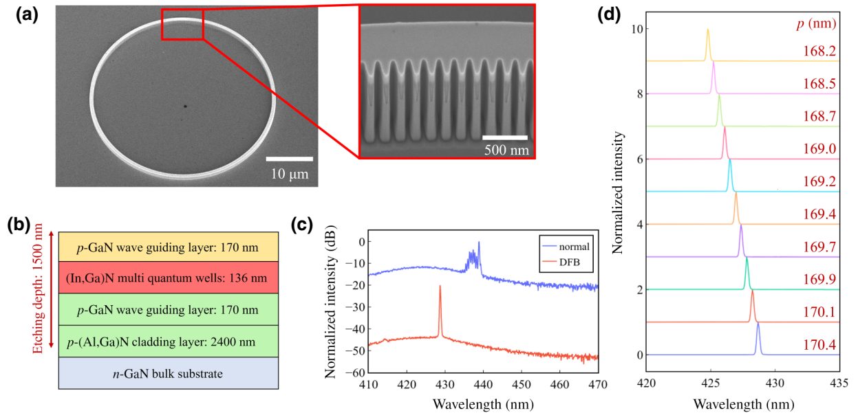
FIG. 1. (a) Scanning electron microscopy images of the DFB ring laser. (b) Epitaxial structure of the GaN microring lasers. (c) Typical lasing spectrum of the ordinary microring laser without grating and the DFB microring laser. Our microring laser has eight longitudinal modes due to the large size of the ring. (d) Controlling the lasing spectra of various DFB ring lasers with various grating periods p .
