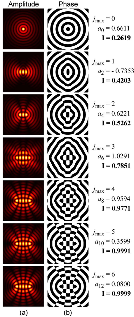
Fig. 2. (Color online) (a) Amplitude and (b) phase of the reconstruction of a \text{MG}_4^e(\xi, \eta; q=25) beam using finite superpositions of BG beams. j_{\max} denotes the number of BG beams used to build up the MG beam.
