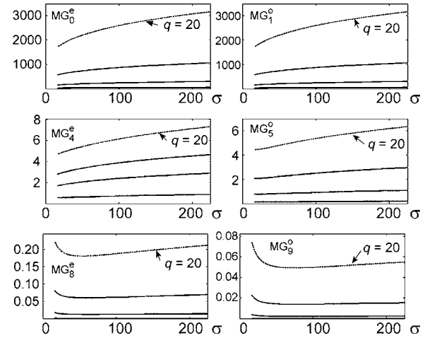
Fig. 1. Behavior of the normalization constants as a function of \sigma for several orders m and q=5, 10, 15, 20 .
