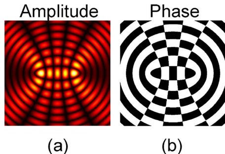
Fig. 3. (Color online) Pure Mathieu nondiffracting beam corresponding to the MG beam shown in Fig. 2.
