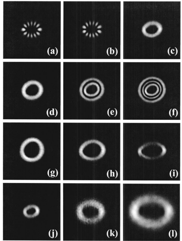
Fig. 2. Experimental intensity results, showing (a) even \text{IG}_{6,6,3} beam, (b) odd \text{IG}_{6,6,3} beam, (c) \text{HIG}_{6,6,3}^+ beam, (d) one intensity ring for the \text{HIG}_{8,8,2}^+ beam, (e) two intensity rings for the \text{HIG}_{10,8,2}^+ beam, (f) three intensity rings for the \text{HIG}_{12,8,2}^+ beam, (g) zero-ellipticity \text{HIG}_{12,12,0}^+ beam, (h) higher ellipticity \text{HIG}_{12,12,6}^+ beam, (i) high ellipticity \text{HIG}_{12,12,12}^+ beam; intensity for the \text{HIG}_{4,4,2}^+ beam at (j) the focal plane, (k) 0.8 m, and (l) 1.0 m. Photographs show 600 \times 600 camera pixels with sizes of 6.7 \mu\text{m} square.
