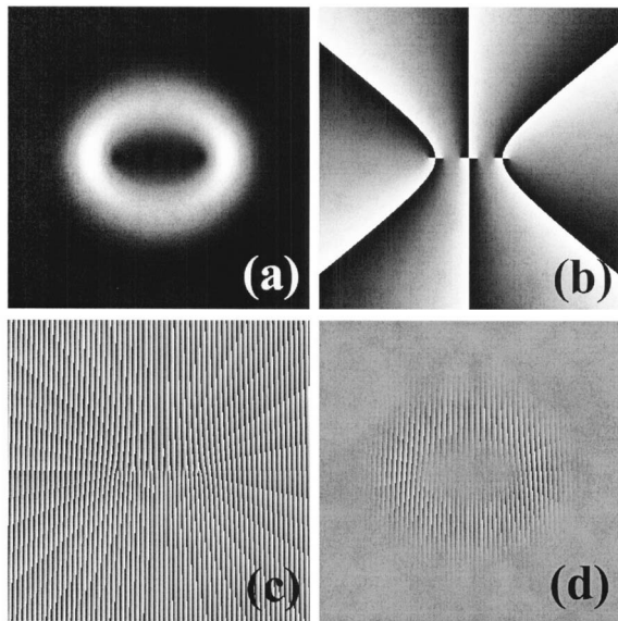
Fig. 1. Computer masks for the \text{HIG}_{6,6,3}^+ beam, showing (a) magnitude, (b) phase, (c) linear phase added to HIG phase, and (d) amplitude-modulated phase mask.
