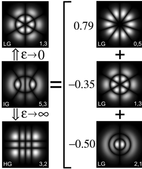
Fig. 3. Left, an IGB tends to a LGB or a HGB when \epsilon \rightarrow 0 or \epsilon \rightarrow \infty , respectively. Right, reconstruction of the even IGB, IG_{5,3}^e = 0.79LG_{0,5}^e - 0.35LG_{1,3}^e - 0.5LG_{2,1}^e .
